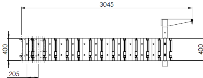
Figure 1: Basic dimensions of JF 100-3.
