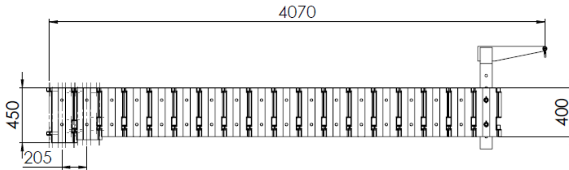
Figure 1: Basic dimensions of JF 100-4.
