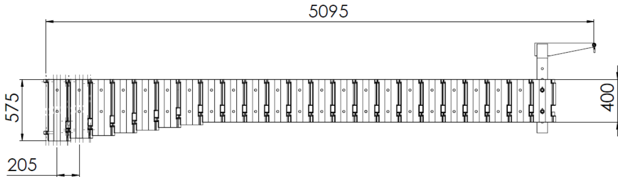
Figure 1: Basic dimensions of JF 100-5.
