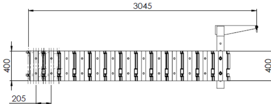
Figure 1: Basic dimensions of JF 150-3.
