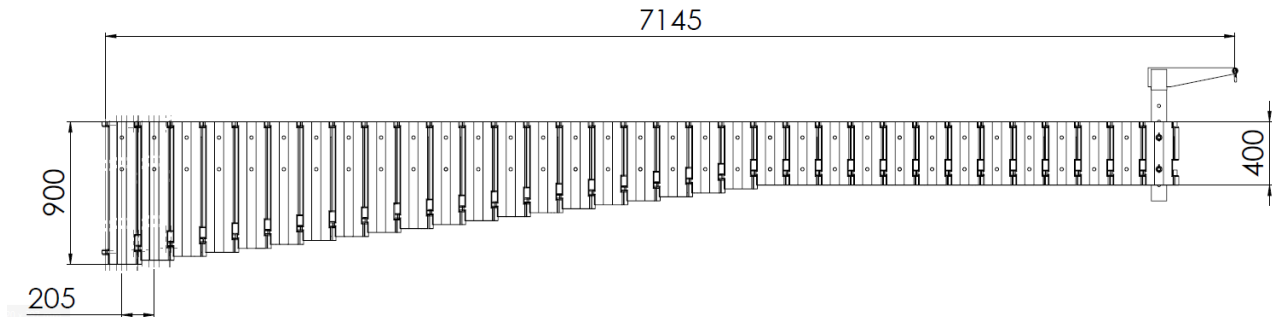
Figure 1: Basic dimensions of JF 150-7.
