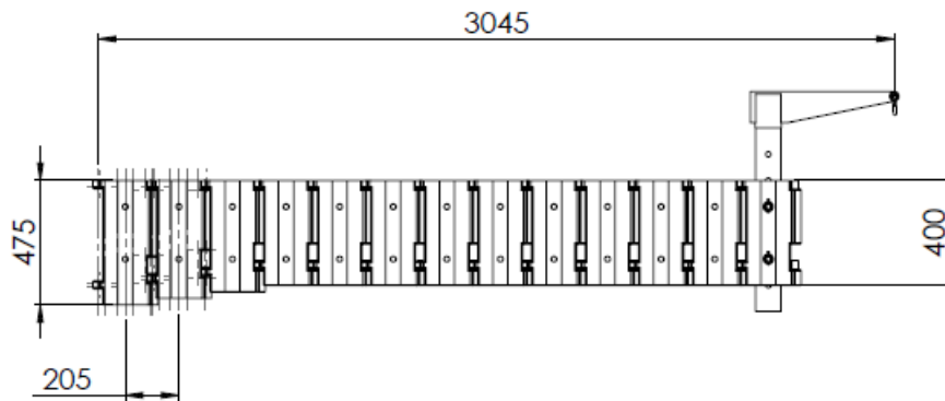
Figure 1: Basic dimensions of JF 200-3.
