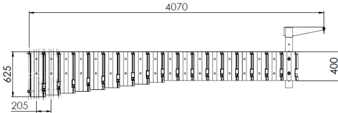
Figure 1: Basic dimensions of JF 200-4.
