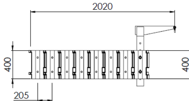
Figure 1: Basic dimensions of JF 250-2.
