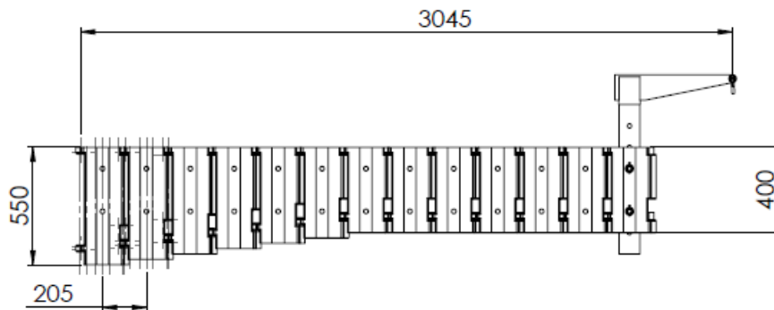
Figure 1: Basic dimensions of JF 250-3.
