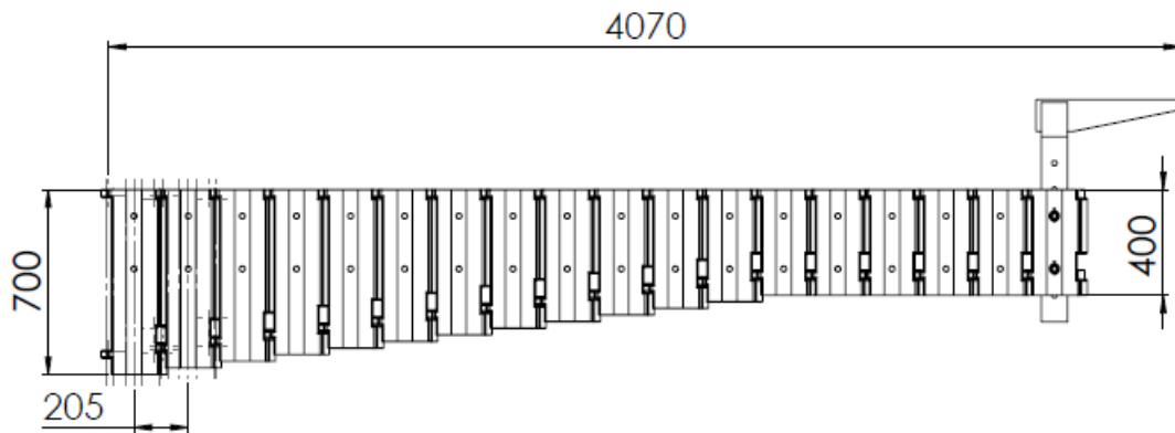
Figure 1: Basic dimensions of JF 250-4.
