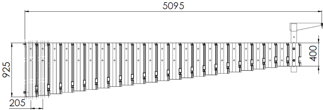
Figure 1: Basic dimensions of JF 250-5.
