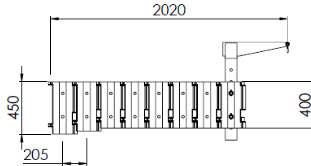
Figure 1: Basic dimensions of JF 300-2.
