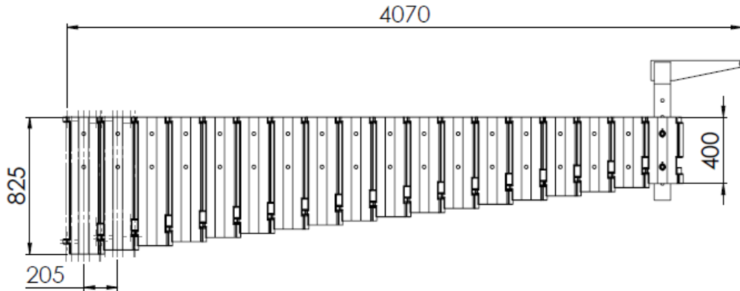
Figure 1: Basic dimensions of JF 300-4.
