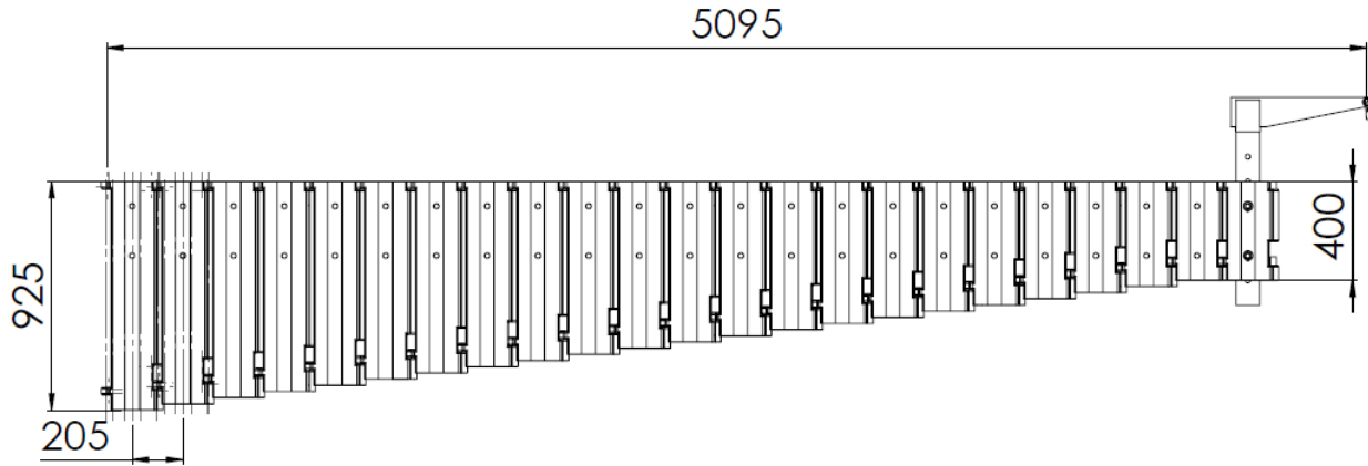
Figure 1: Basic dimensions of JF 300-5.
