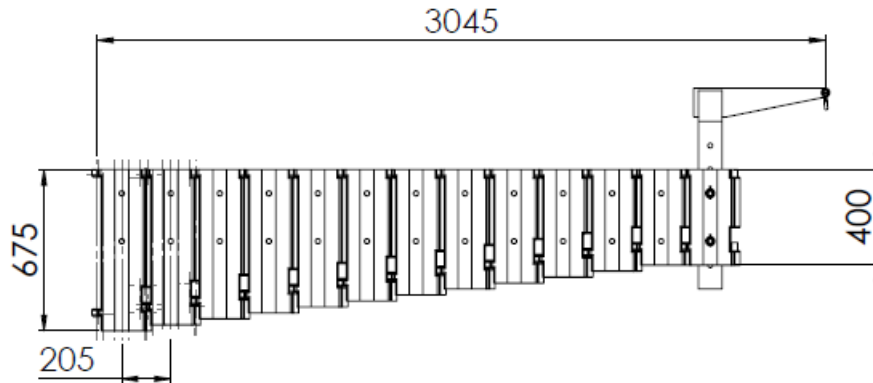
Figure 1: Basic dimensions of JF 350-3.
