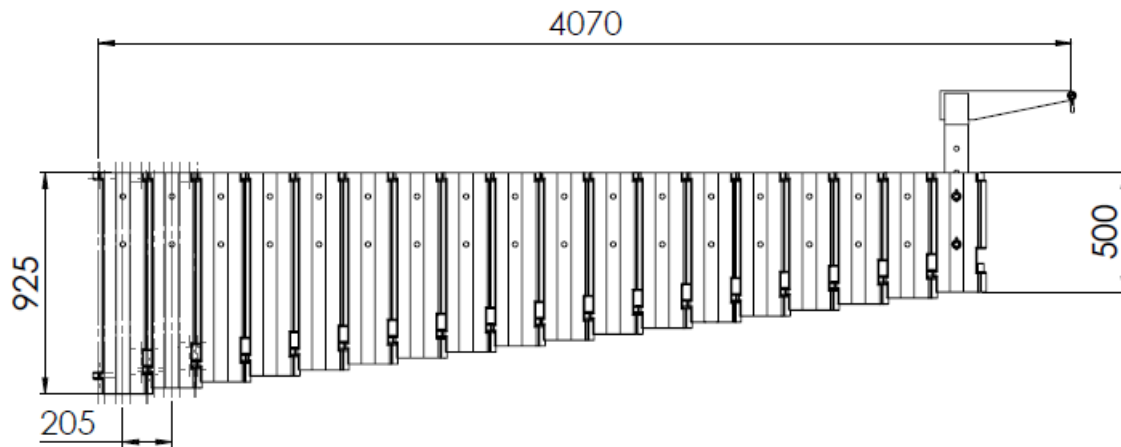
Figure 1: Basic dimensions of JF 350-4.
