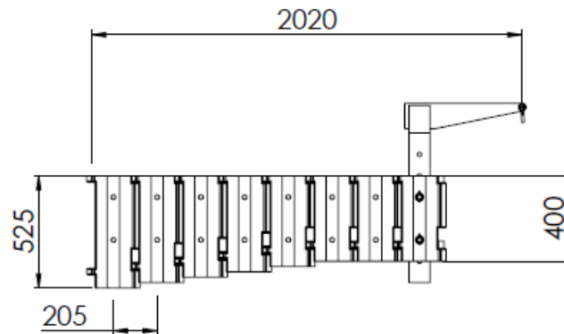
Figure 1: Basic dimensions of JF 400-2.
