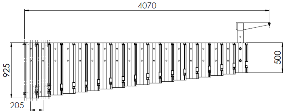
Figure 1: Basic dimensions of JF 400-4.
