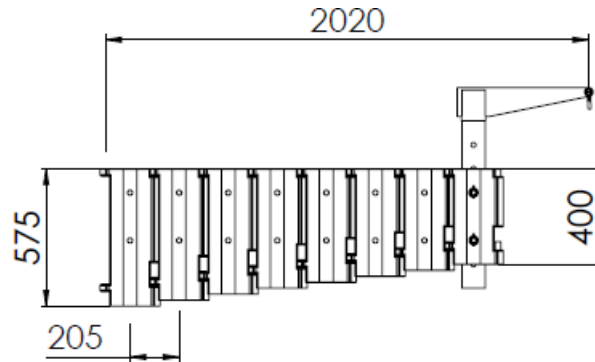
Figure 1: Basic dimensions of JF 450-2.
