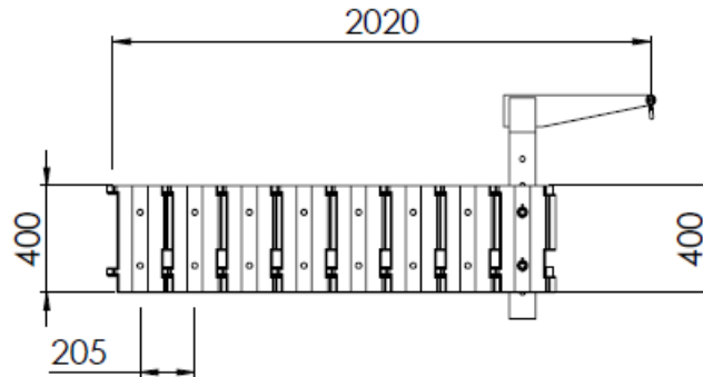
Figure 1: Basic dimensions of JF 50-2.
