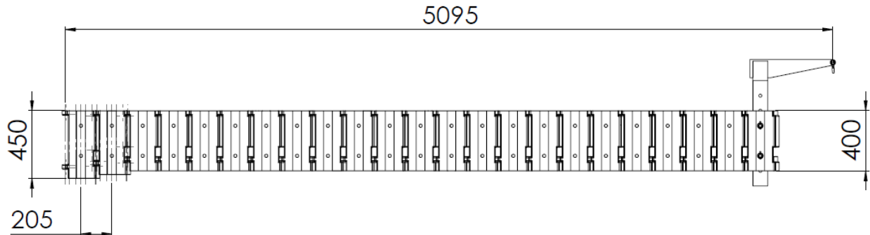
Figure 1: Basic dimensions of JF 50-5.
