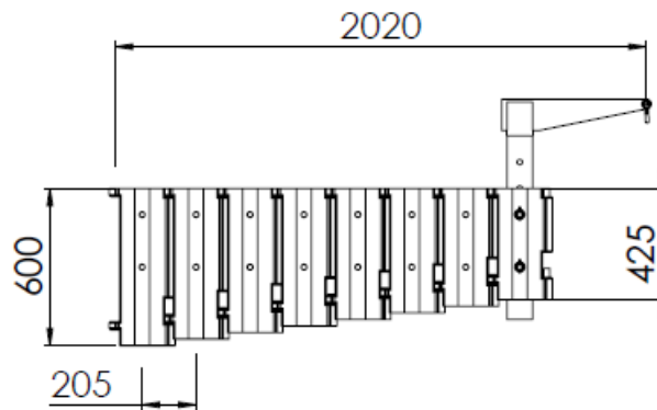
Figure 1: Basic dimensions of JF 500-2.
