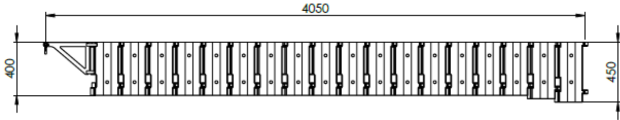
Figure 1: Basic dimensions of JF 100-4.
