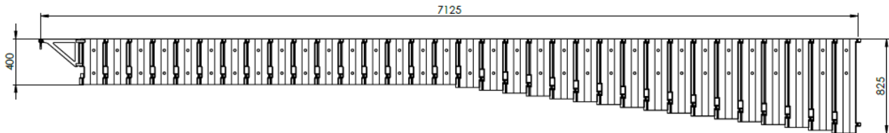
Figure 1: Basic dimensions of JF 100-7.
