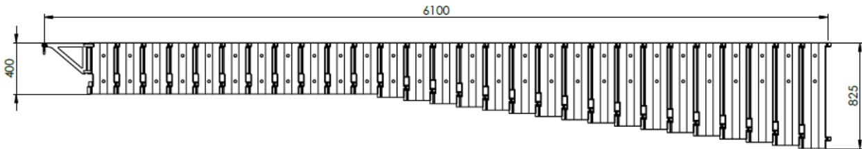
Figure 1: Basic dimensions of JF 150-6.
