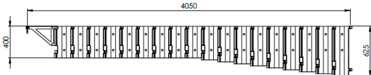
Figure 1: Basic dimensions of JF 200-4.
