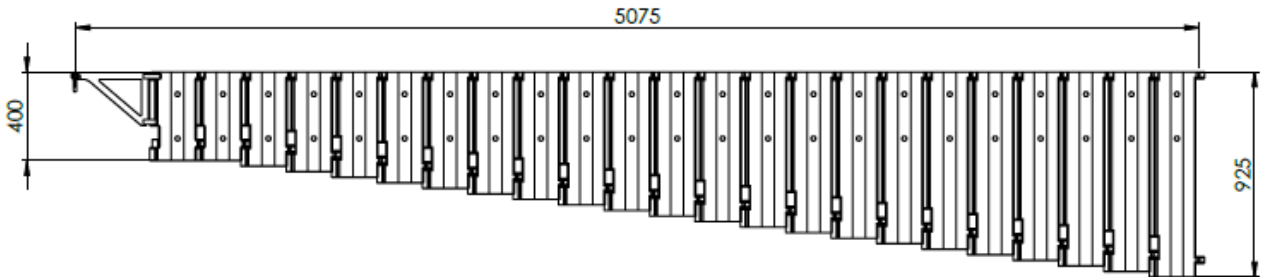
Figure 1: Basic dimensions of JF 250-5.
