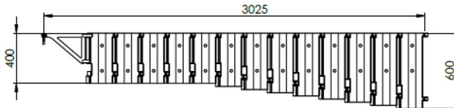
Figure 1: Basic dimensions of JF 300-3.
