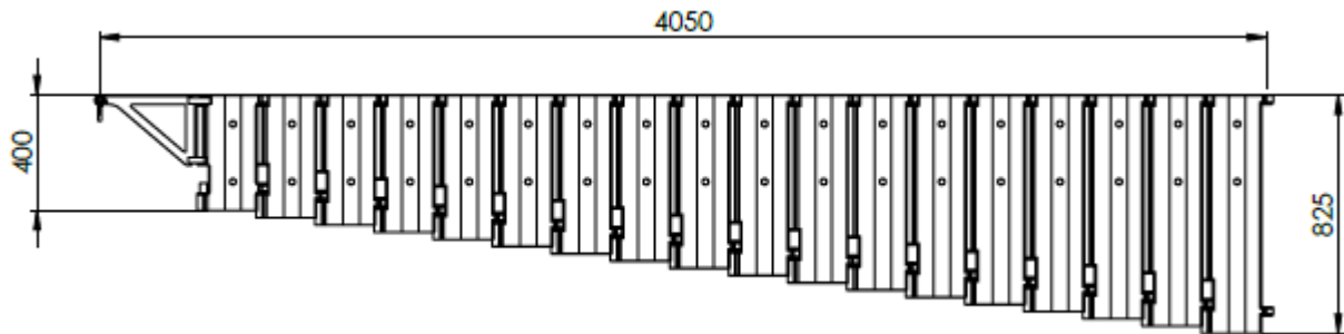
Figure 1: Basic dimensions of JF 300-4.
