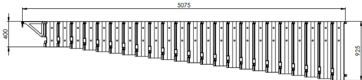
Figure 1: Basic dimensions of JF 300-5.
