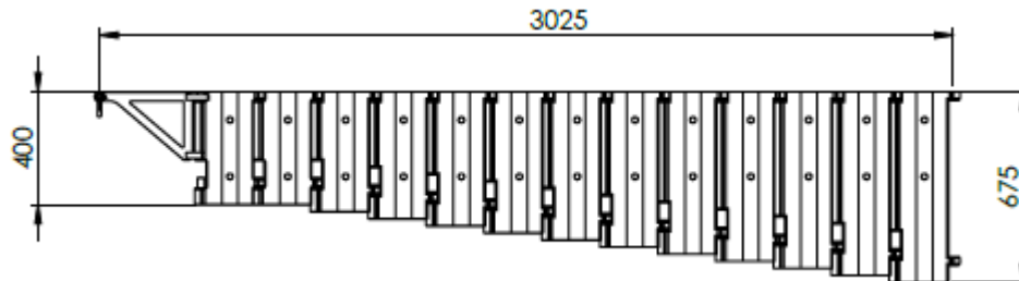
Figure 1: Basic dimensions of JF 350-3.
