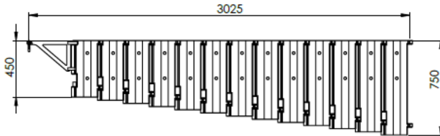
Figure 1: Basic dimensions of JF 400-3.
