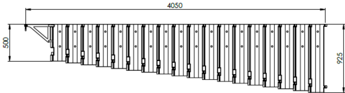
Figure 1: Basic dimensions of JF 400-4.
