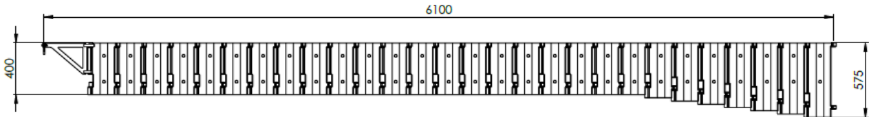
Figure 1: Basic dimensions of JF 50-6.
