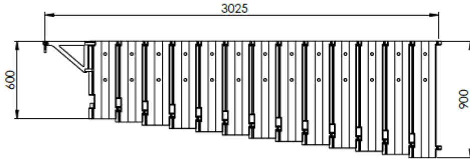
Figure 1: Basic dimensions of JF 500-3.
