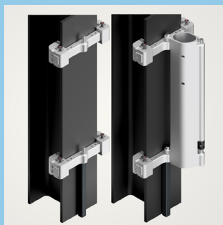
H-beam brackets
